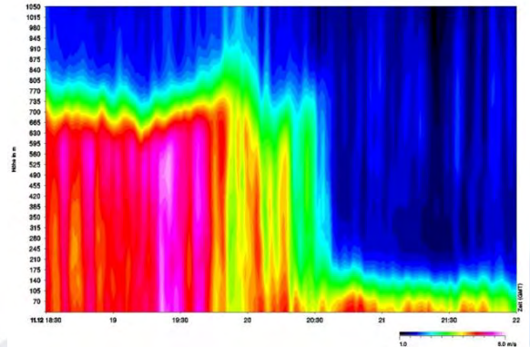
Time height cross sections during a rain event with melting zone
