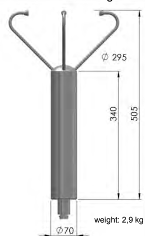
Mechanical drawing
